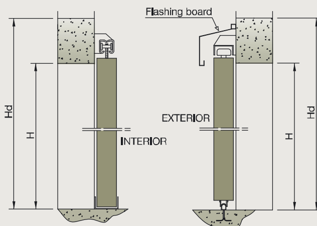
Vertical sections
